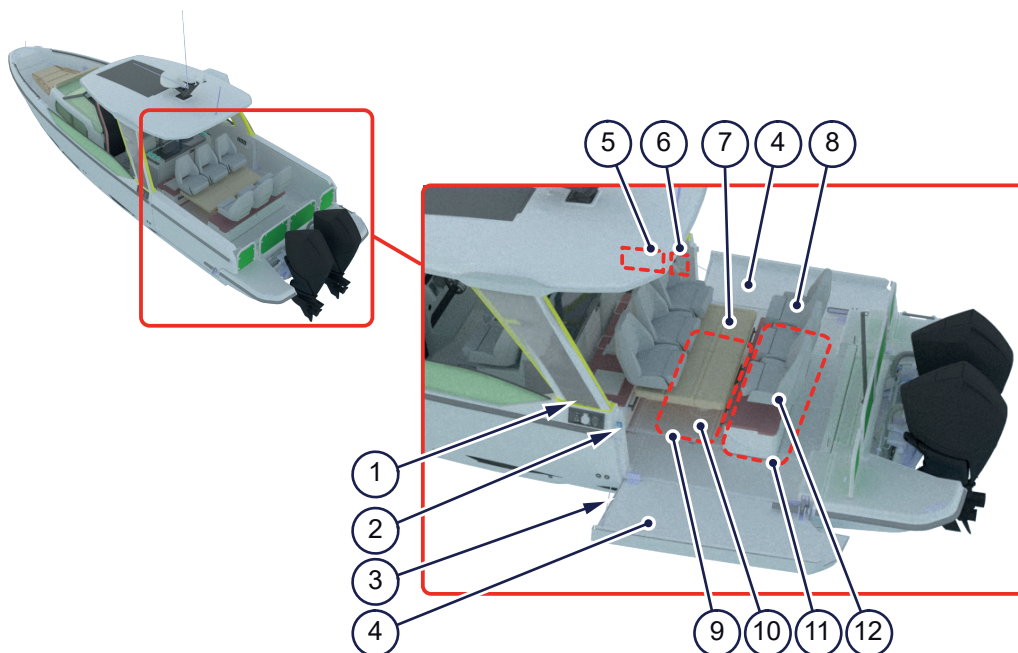
Figure 4.5 - Aft deck
