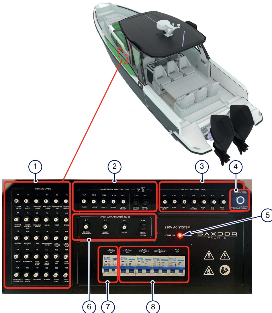
Figure 4.14 - Fuse panel
