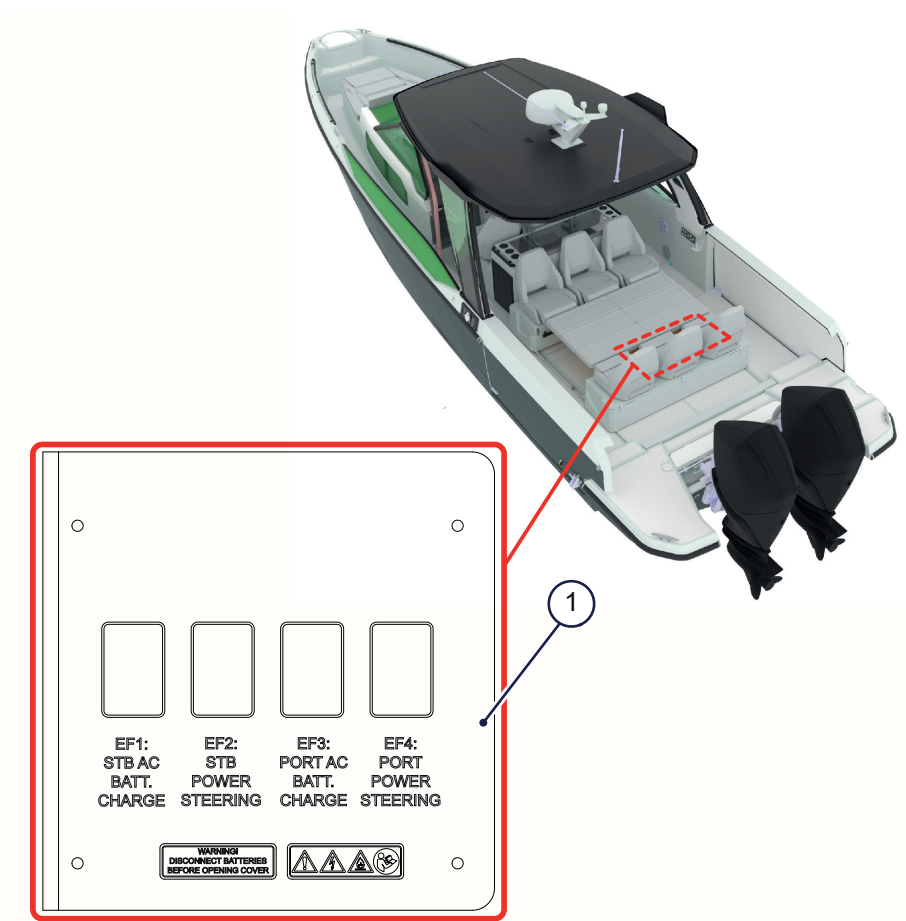
Figure 4.15 - Heavy-duty fuse panel
