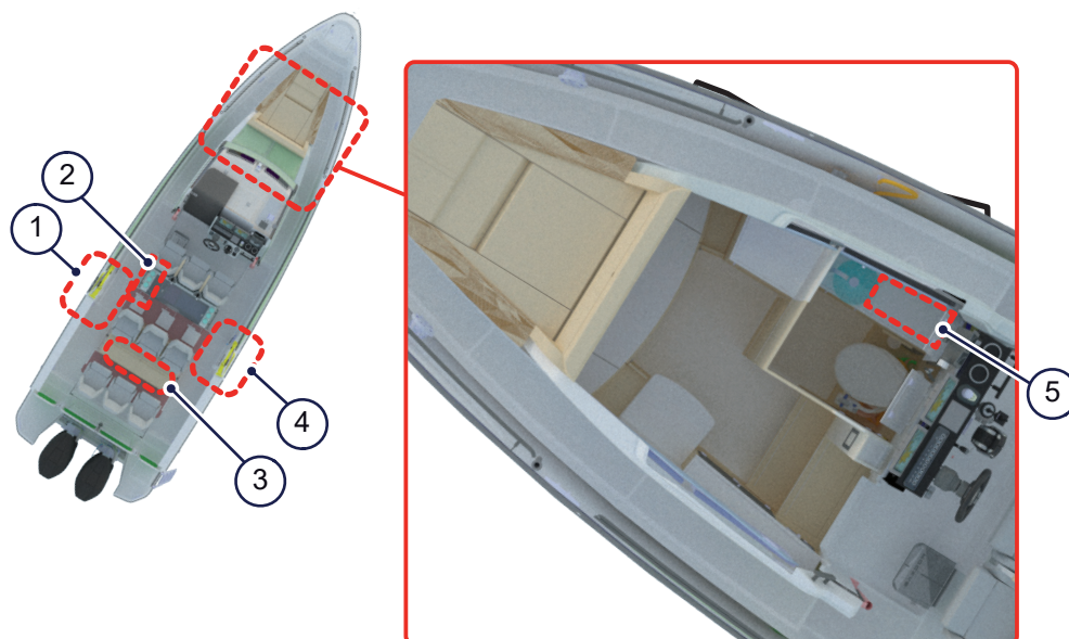
Figure 4.28 - Seacocks
