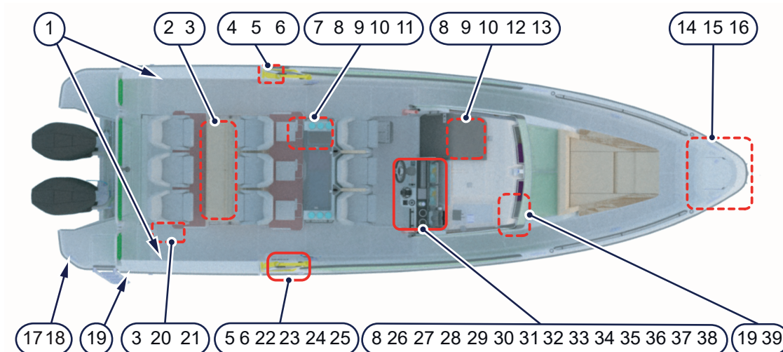
Figure 4.23 - Location of safety labels on your boat
