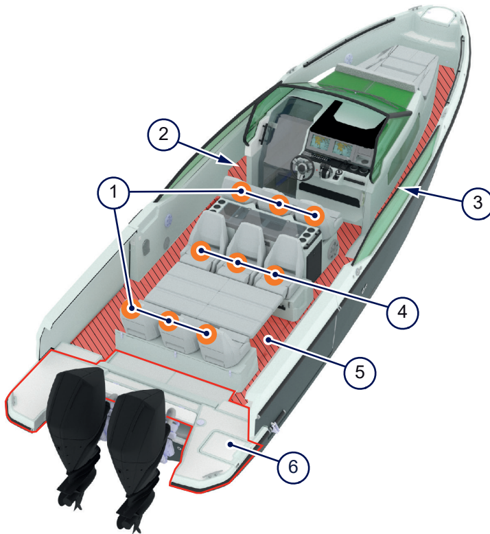
Figure 4.22 - Safe seating and moving areas
