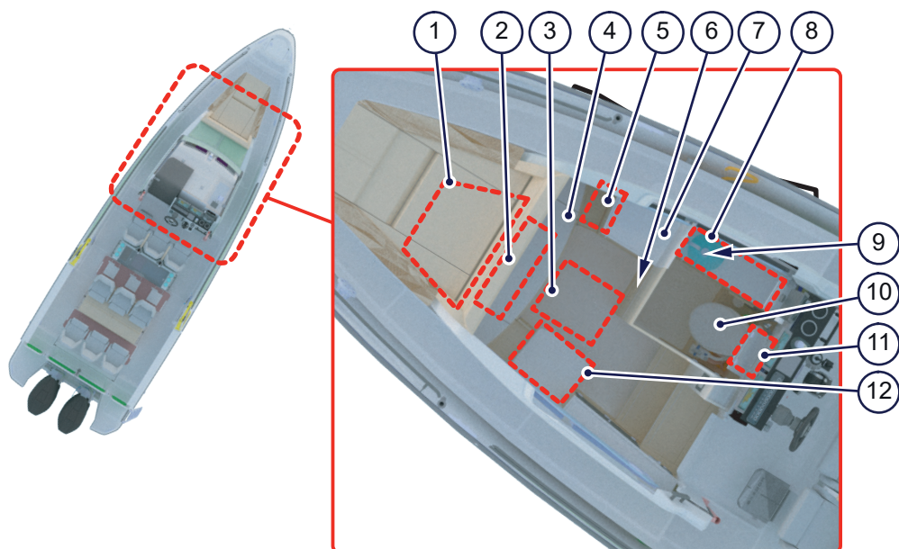
Figure 4.3 - Front cabin
