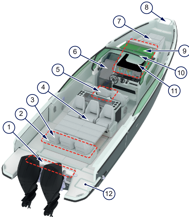
Figure 4.27 - Hatches
