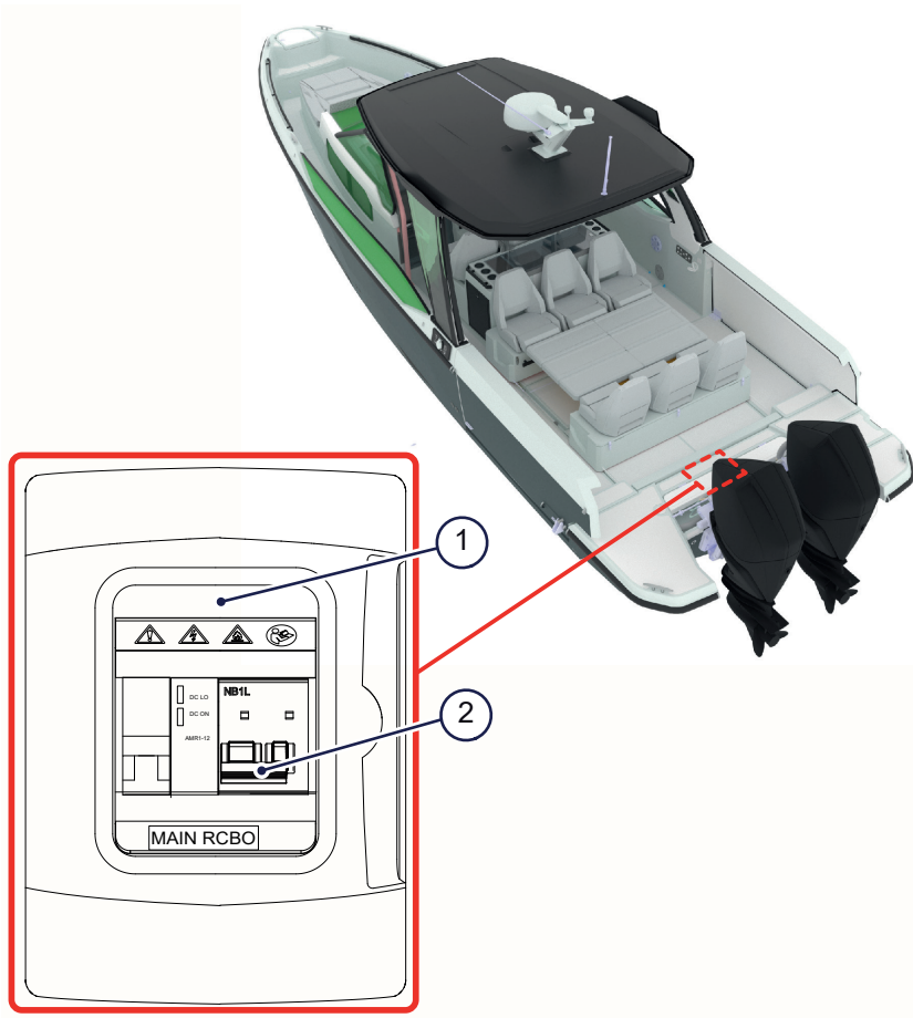
Figure 4.16 - Air-conditioning fuse panel
