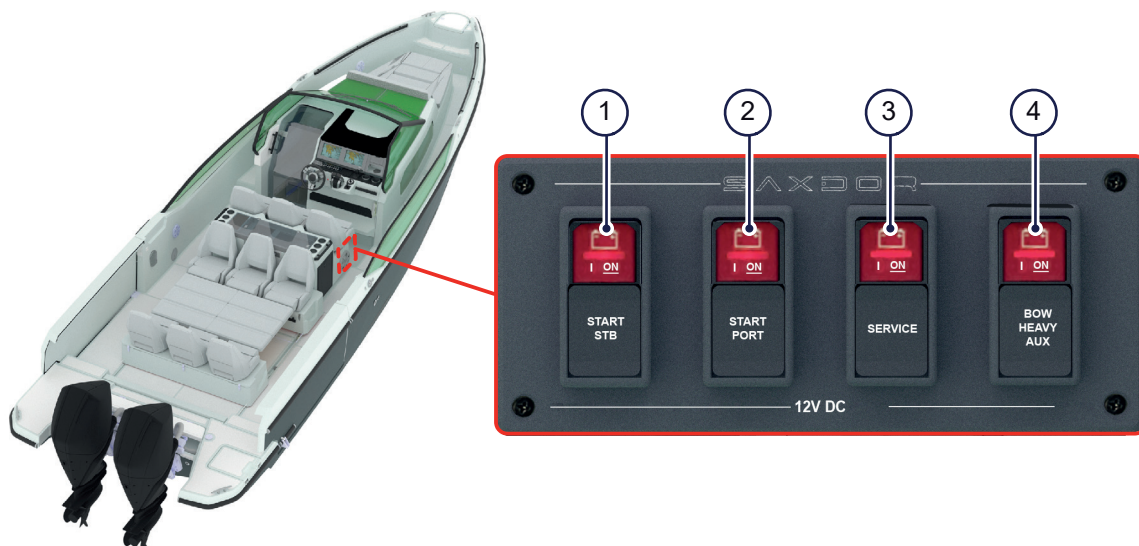
Figure 4.17 - Battery control panel
