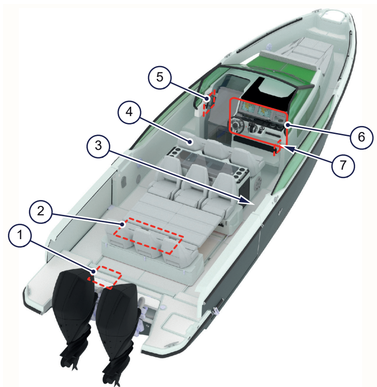
Figure 4.7 - Locations of user controls
