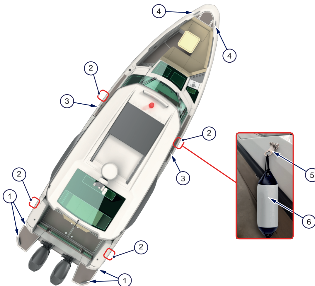
Figure 4.24 - Attachment points
