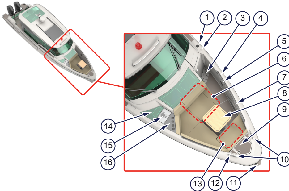
Figure 4.2 - Foredeck
