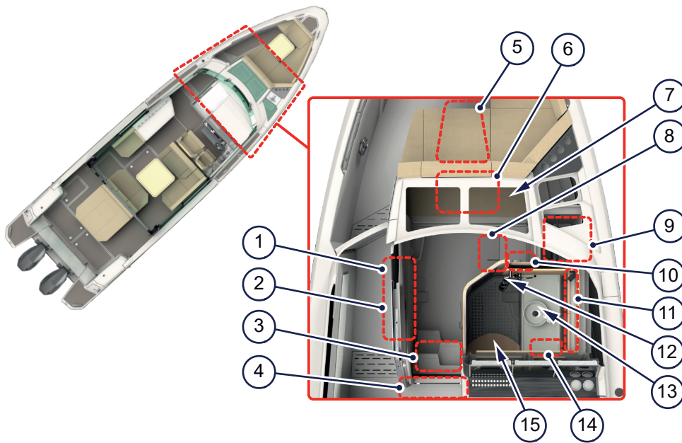
Figure 4.3 - Front cabin
