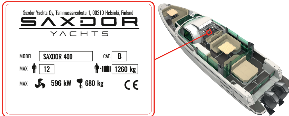
Figure 4.20 - Builder's plate
