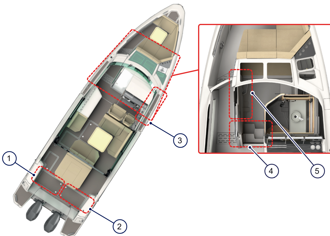
Figure 4.29 - Seacocks
