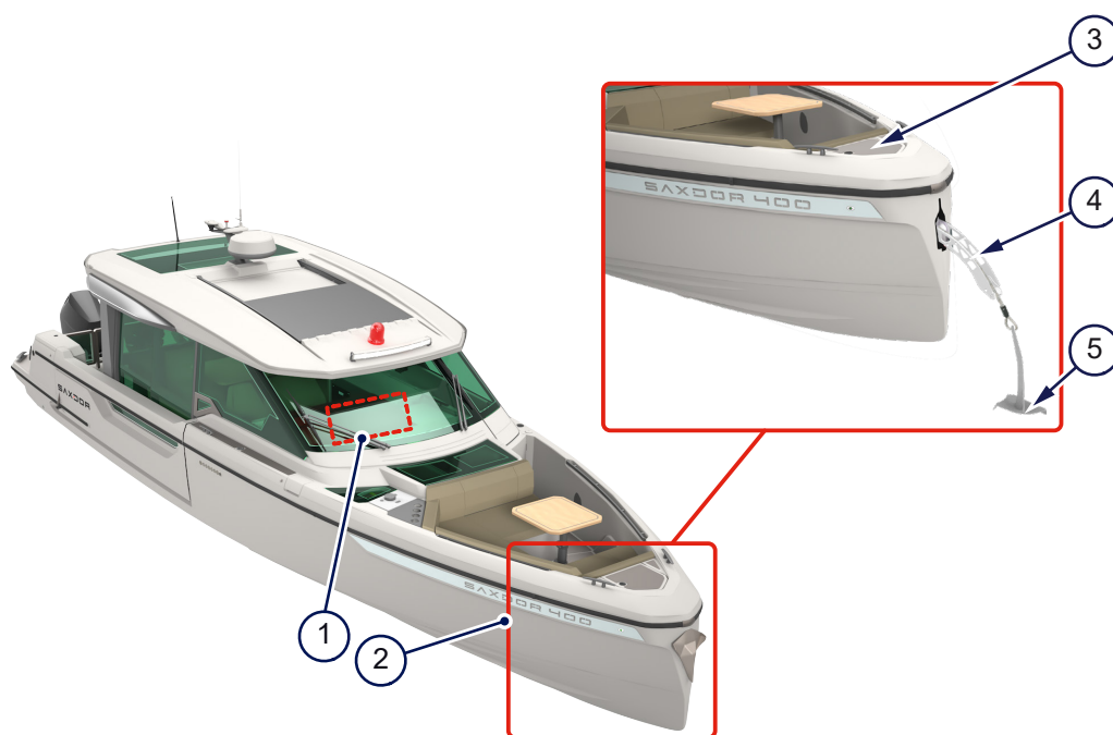
Figure 5.10 - Anchor system
