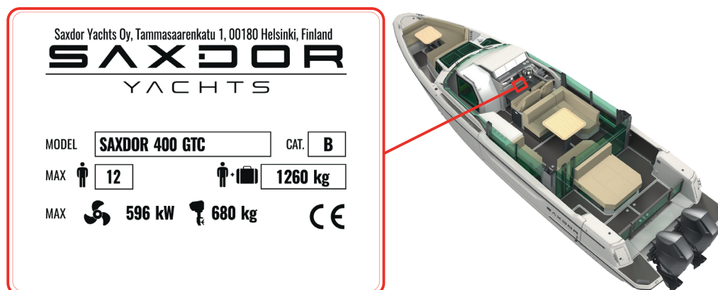
Figure 4.21 - Builder's plate
