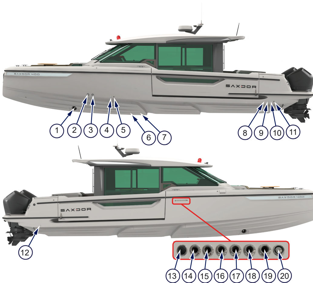
Figure 4.27 - Hull openings
