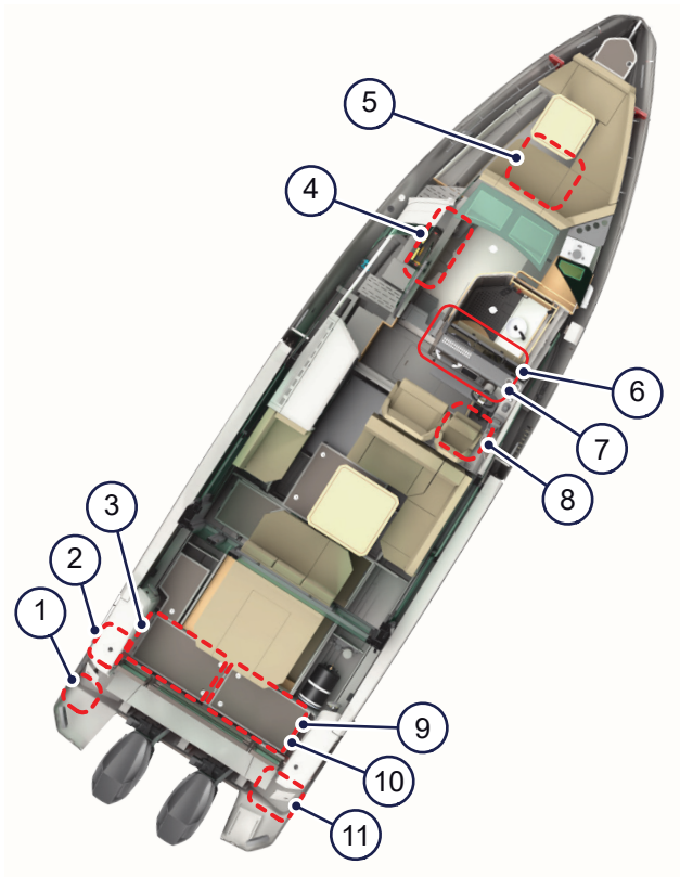
Figure 5.1 - Electrical system
