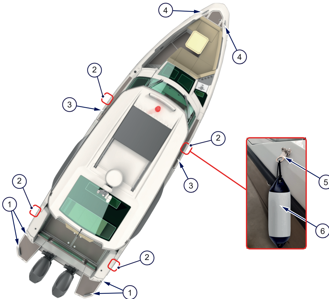
Figure 4.25 - Attachment points
