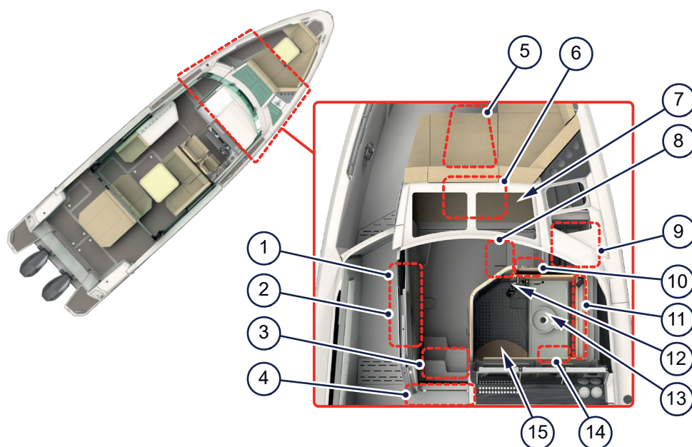
Figure 4.3 - Front cabin
