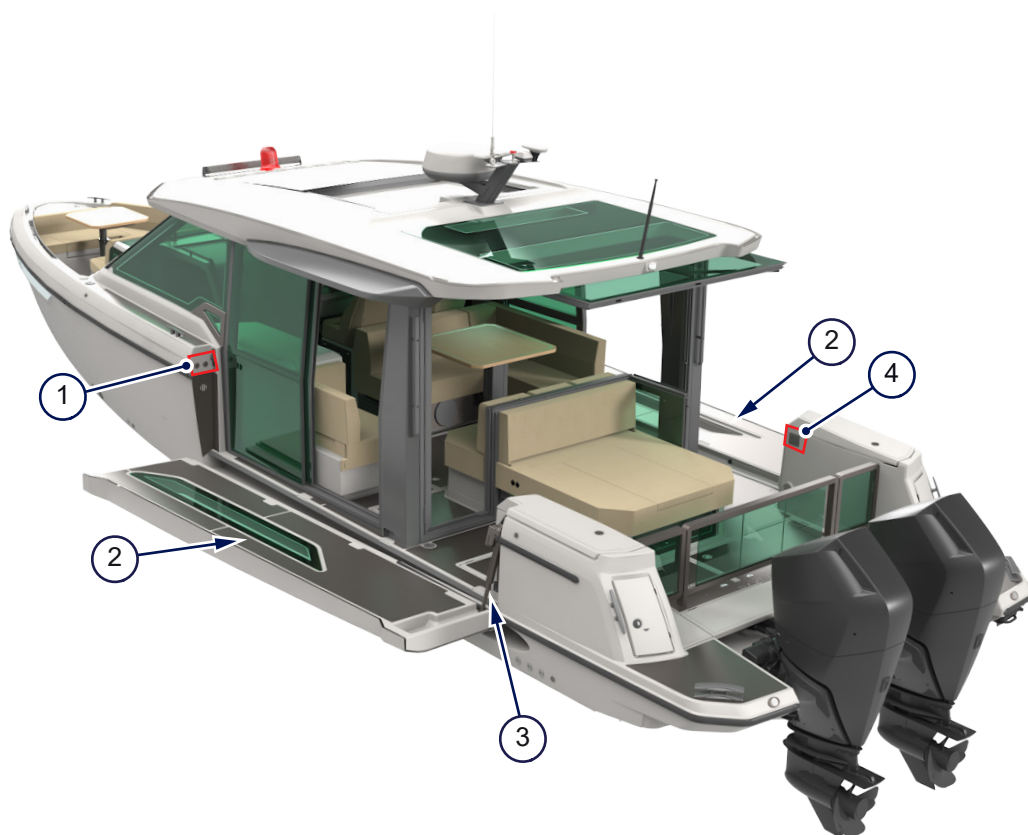
Figure 5.12 - Side terraces
