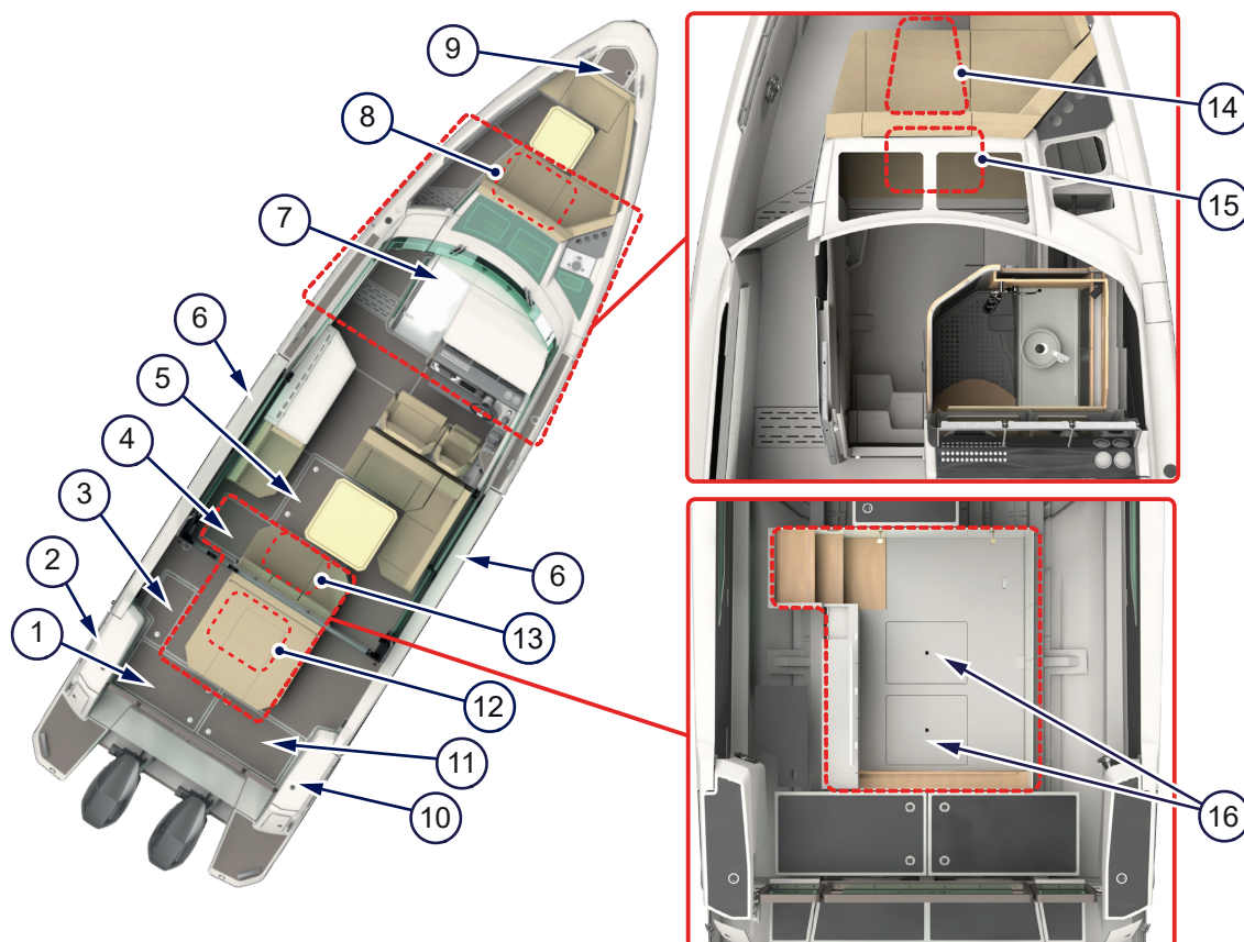
Figure 4.28 - Hatches
