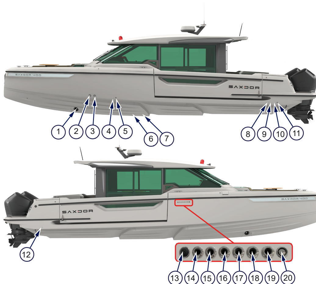
Figure 4.27 - Hull openings
