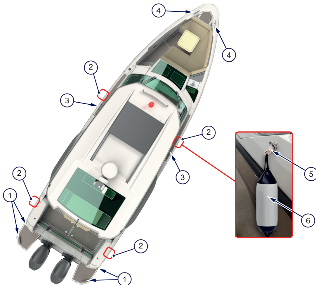
Figure 4.25 - Attachment points
