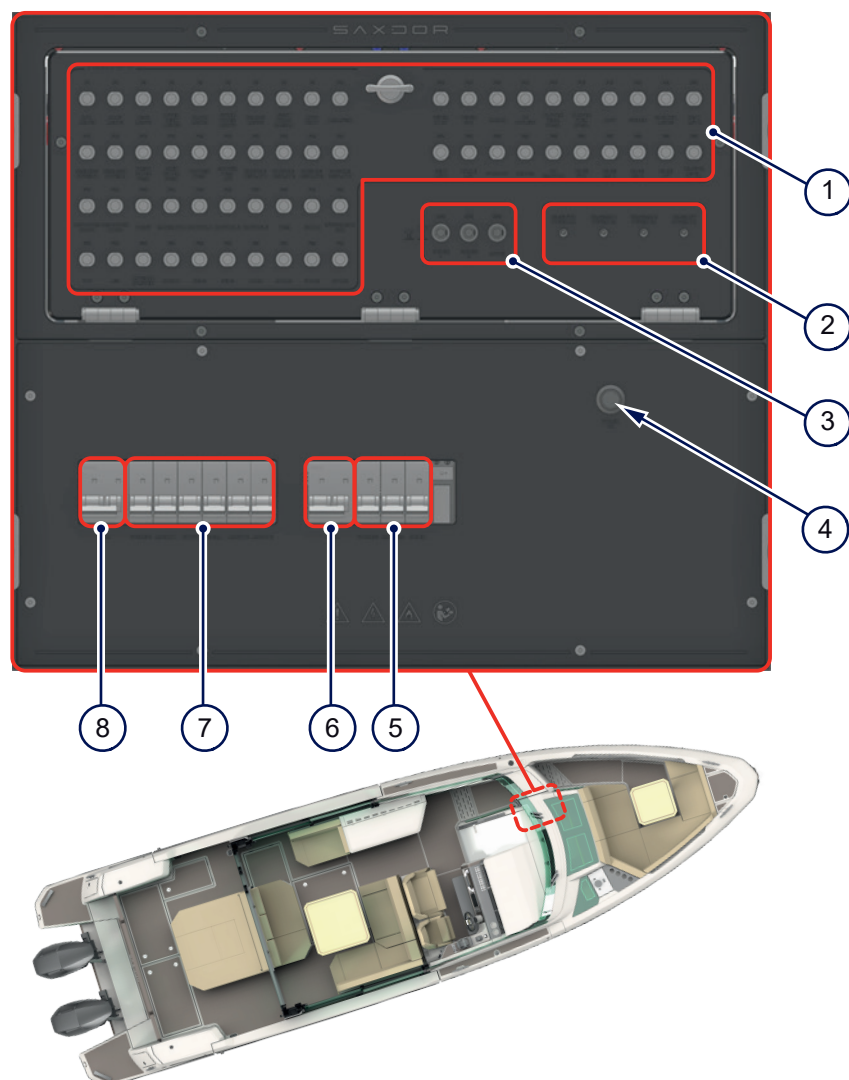
Figure 4.15 - Fuse panel
