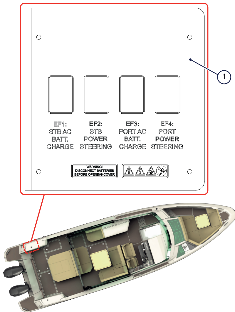
Figure 4.16 - Heavy-duty fuse panel
