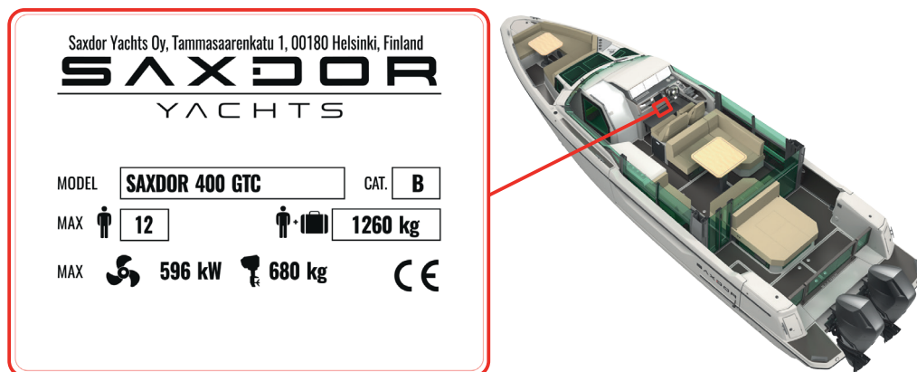
Figure 4.21 - Builder's plate
