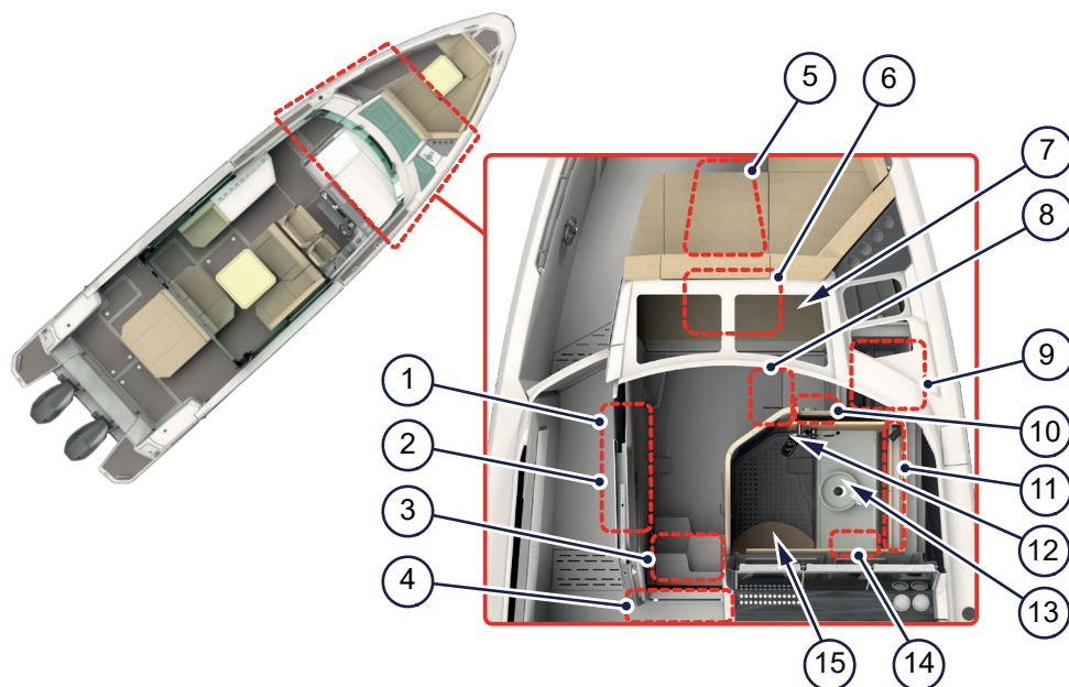
Figure 4.3 - Front cabin
