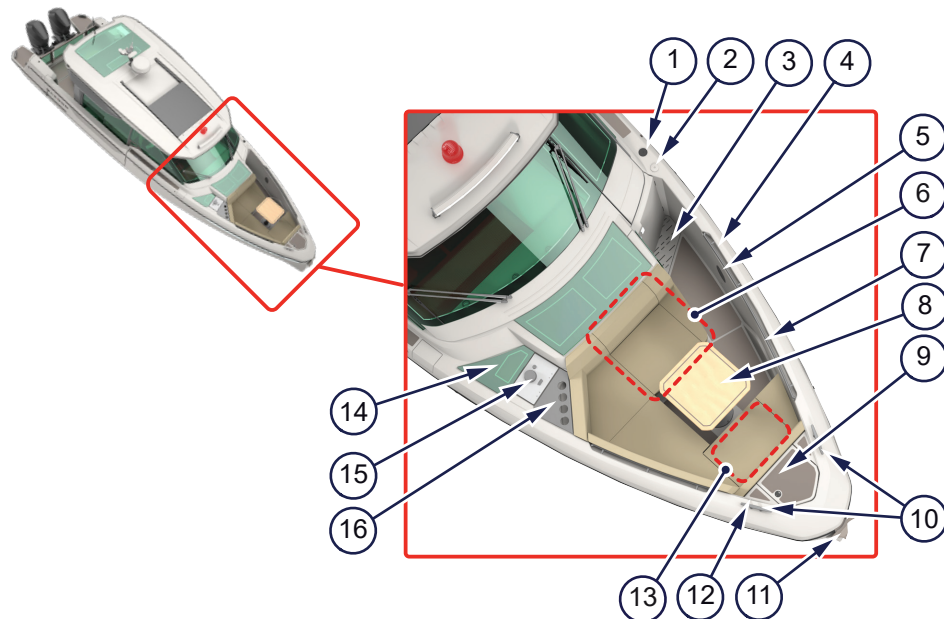
Figure 4.2 - Foredeck
