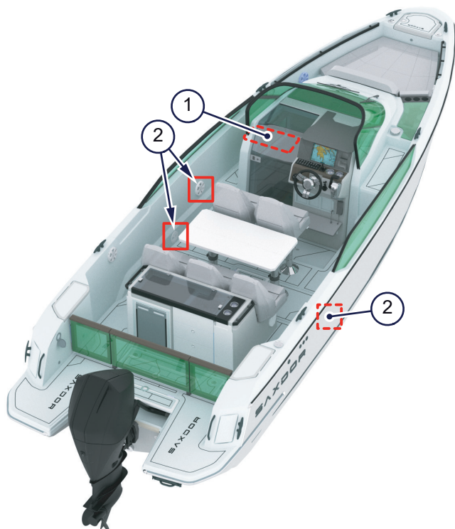
Figure 4.23 - Seacocks
