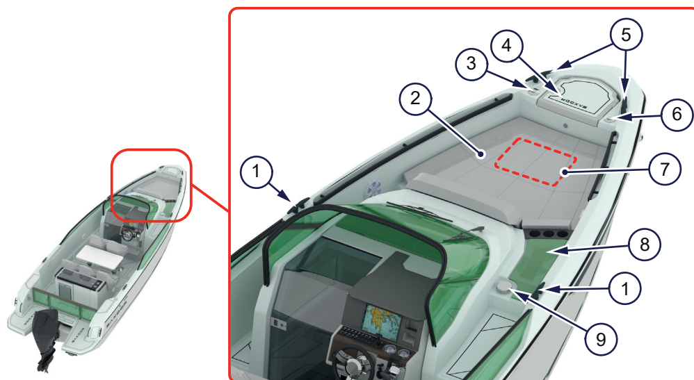
Figure 4.2 - Foredeck
