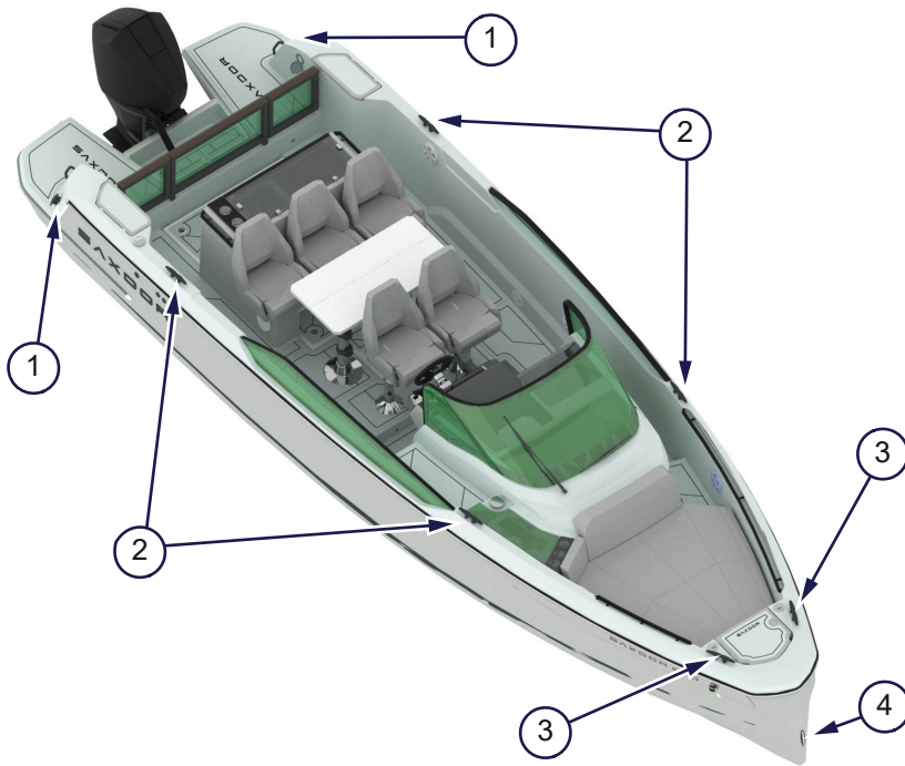
Figure 4.19 - Attachment points
