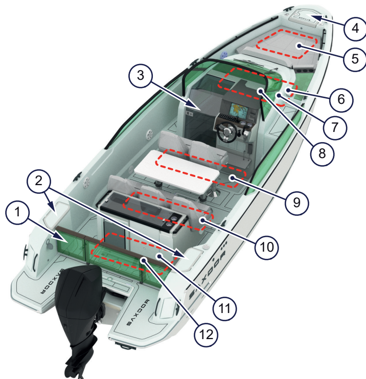
Figure 4.22 - Hatches
