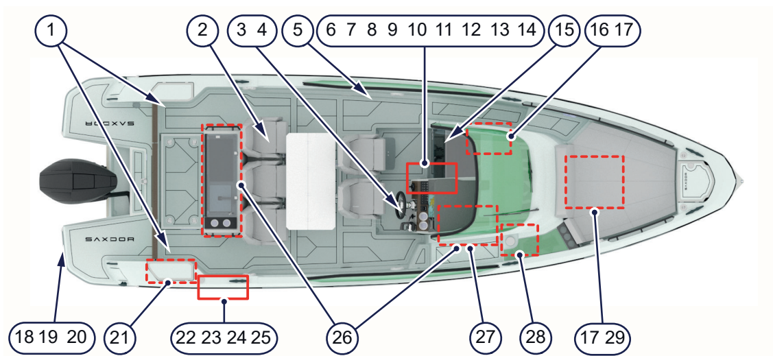
Figure 4.18 - Location of safety labels on your boat
