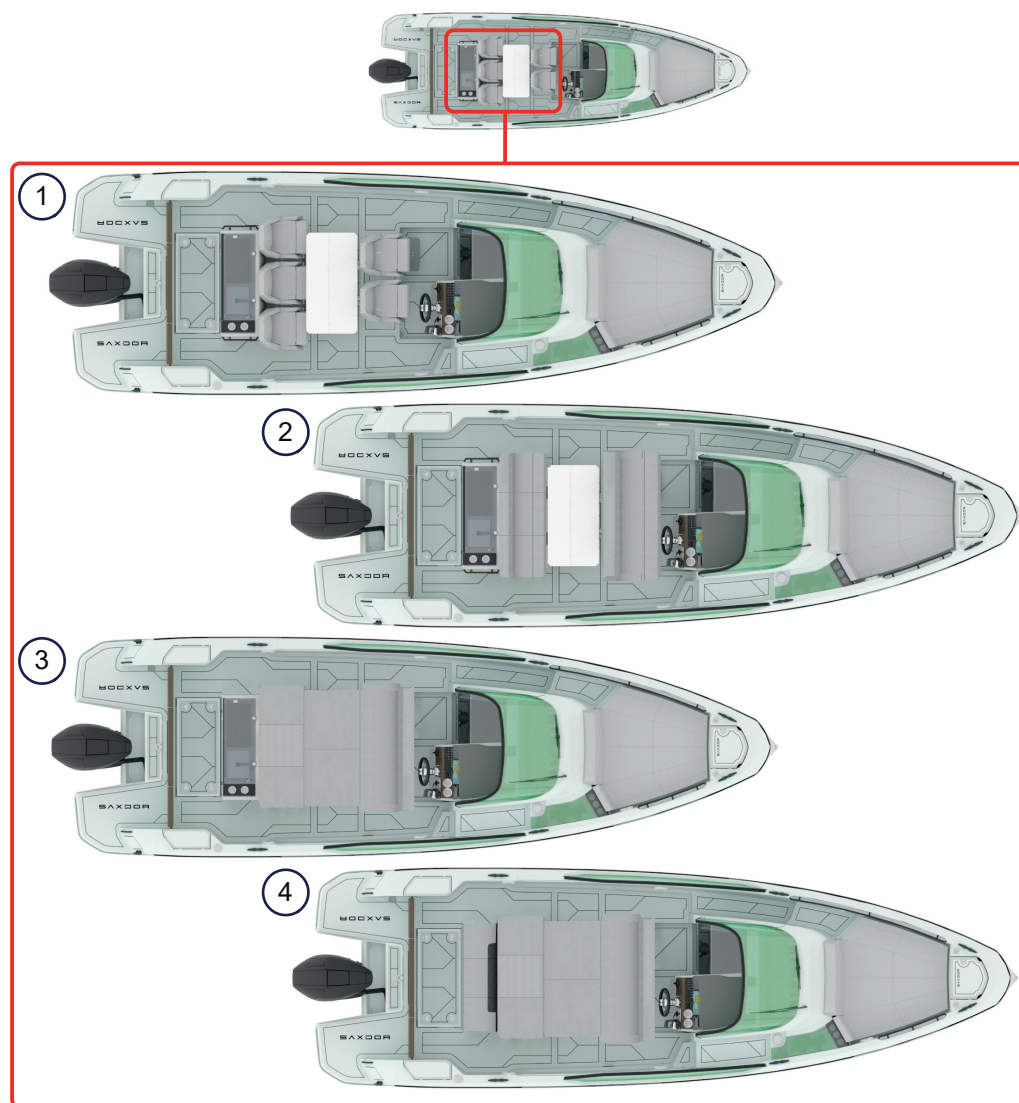
Figure 5.9 - Seating setups
