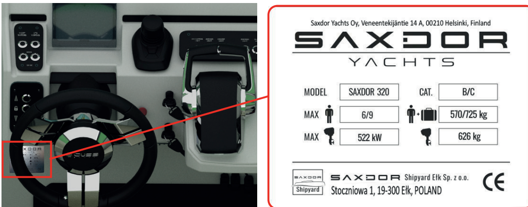
Figure 4.20 - Builder's plate
