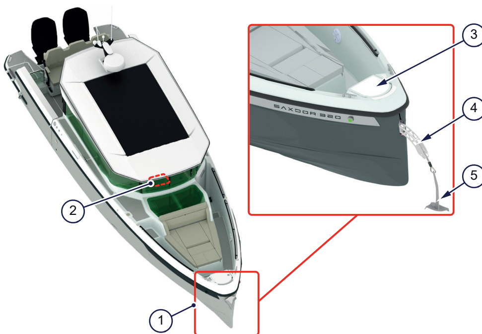
Figure 5.8 - Anchor system
