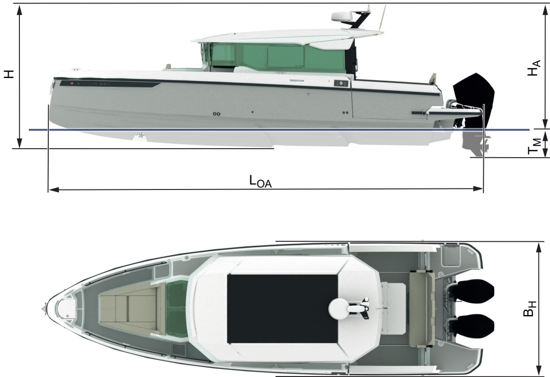
Figure 8.1 - Saxdor 320 GTC dimensions
