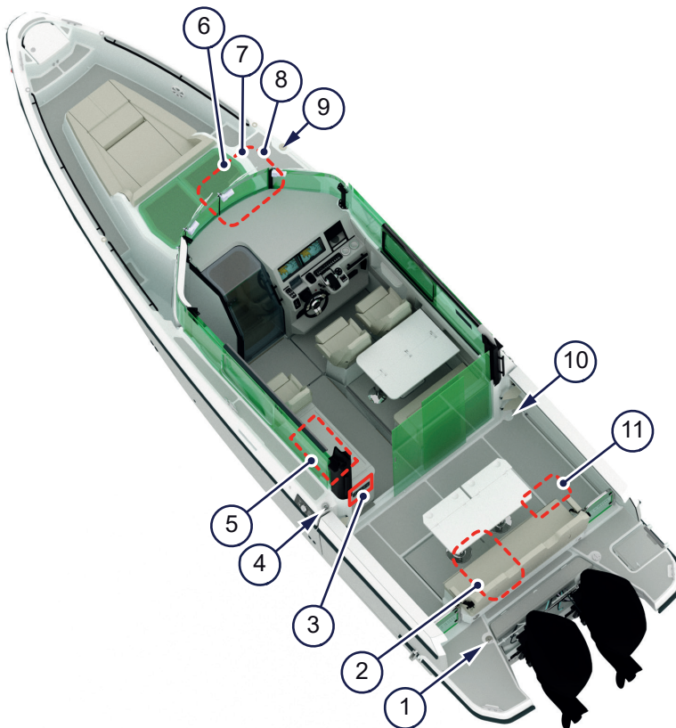
Figure 5.6 - Fresh, grey and black water systems
