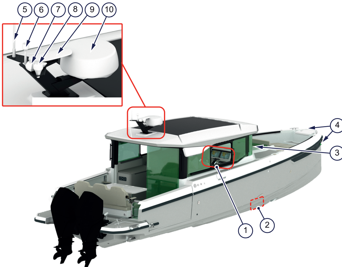
Figure 5.7 - Navigation equipment
