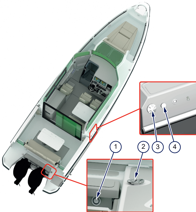
Figure 5.3 - Fuel system
