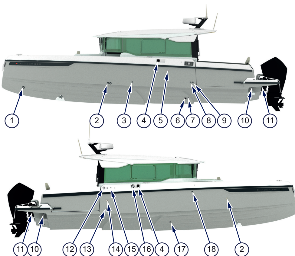
Figure 4.26 - Hull openings
