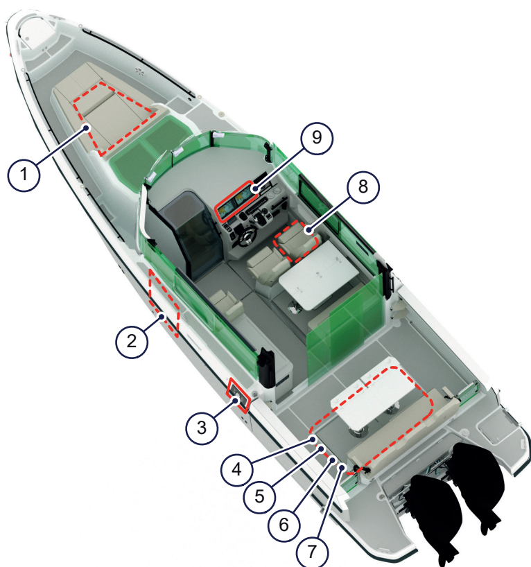
Figure 5.1 - Electrical system
