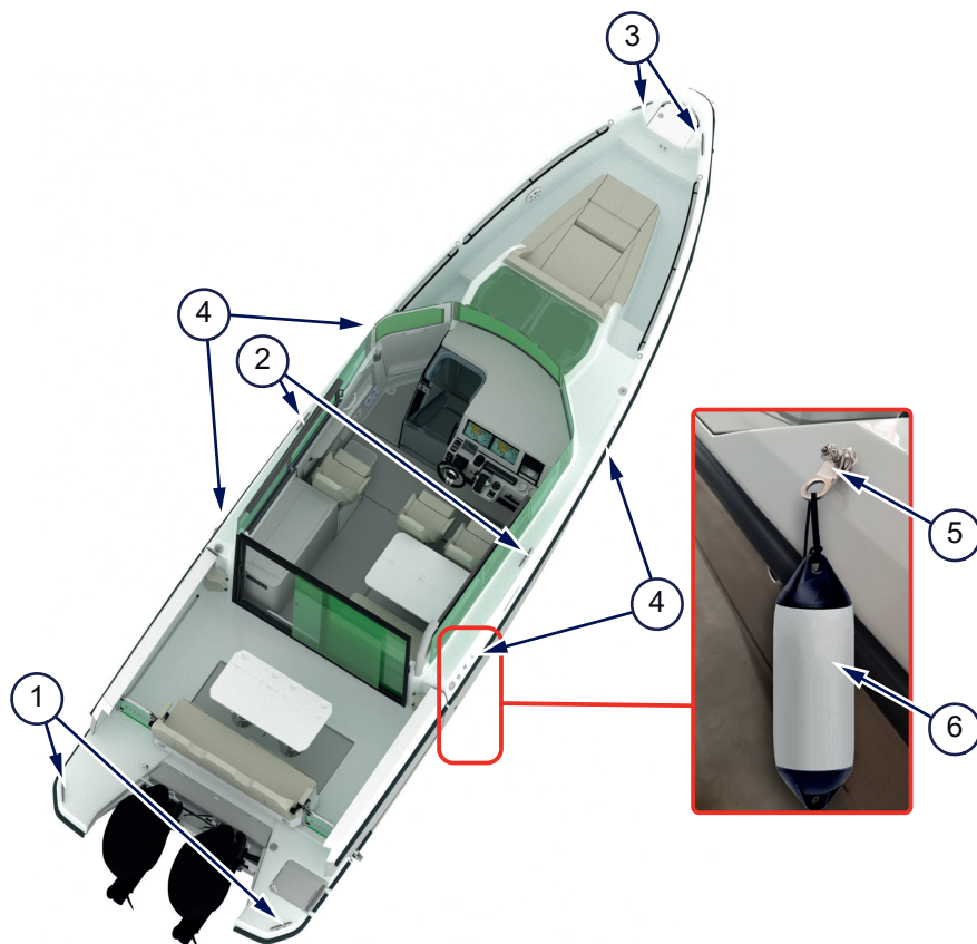
Figure 4.25 - Attachment points
