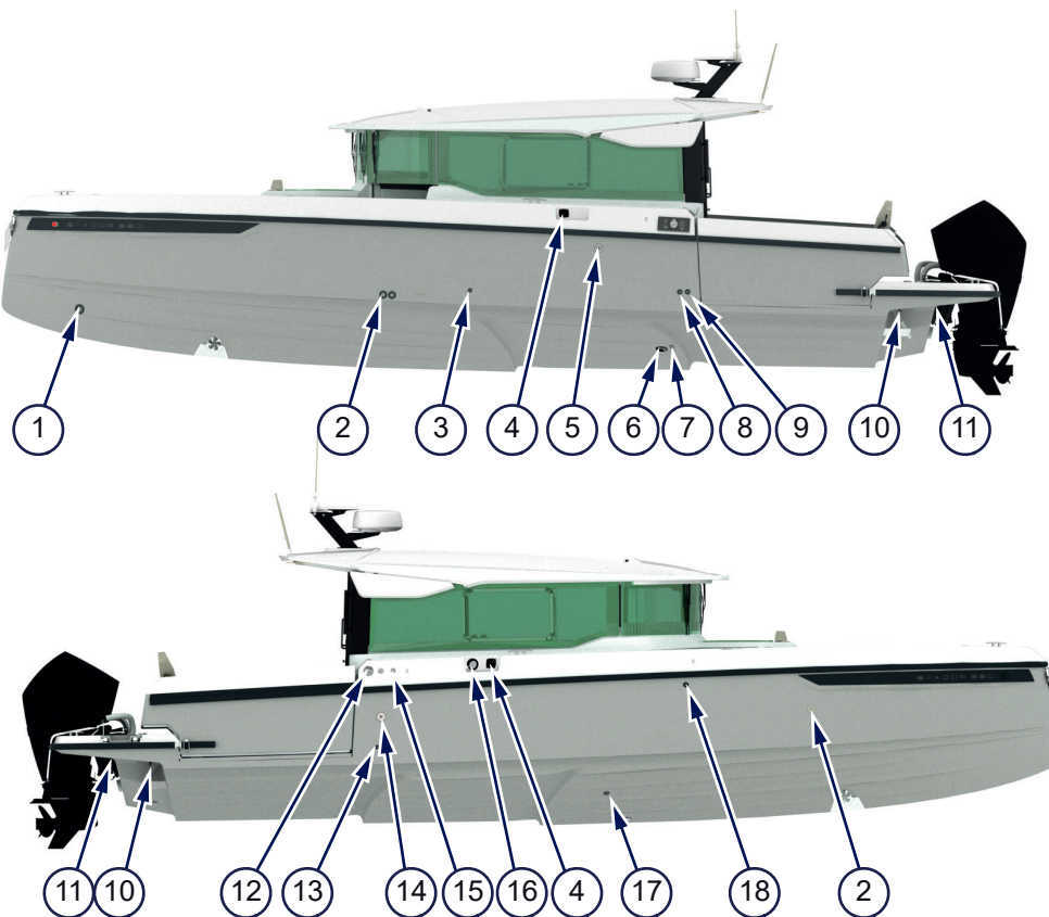
Figure 4.27 - Hull openings
