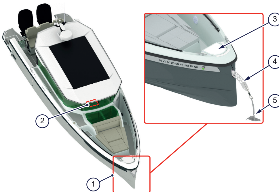
Figure 5.10 - Anchor system
