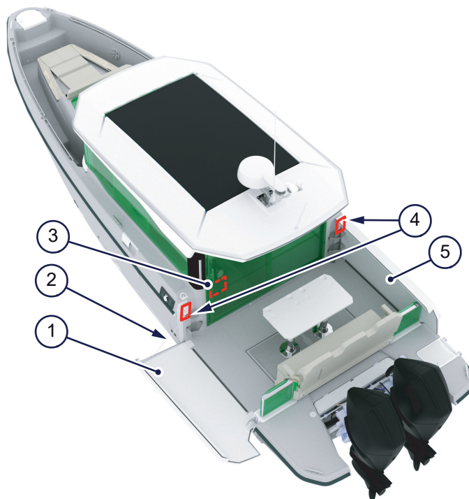
Figure 5.12 - Side terraces
