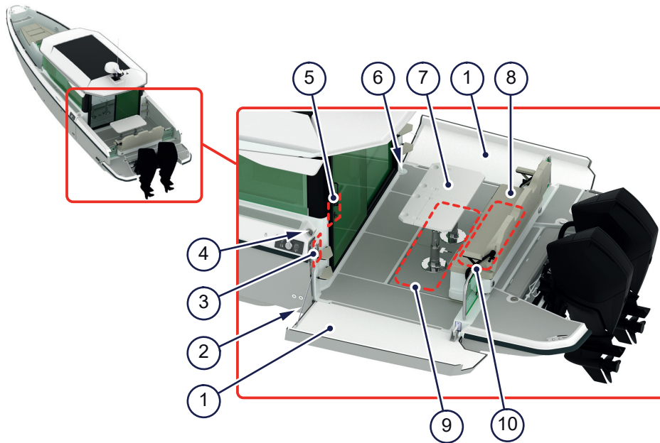
Figure 4.5 - Aft deck
