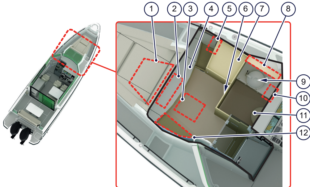
Figure 4.3 - Front cabin
