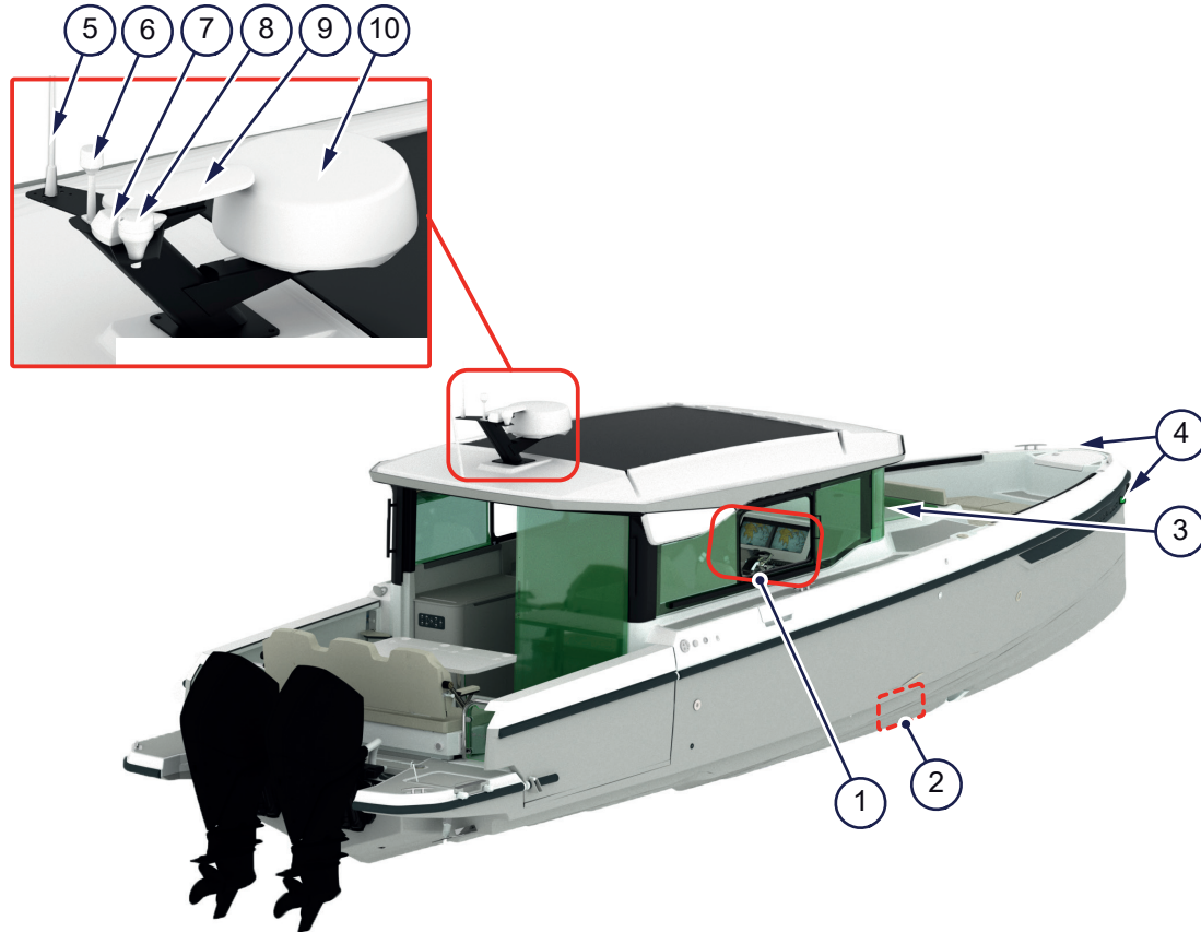
Figure 5.9 - Navigation equipment
