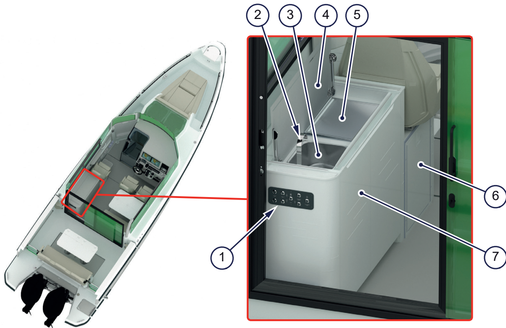
Figure 5.11 - Wet bar
