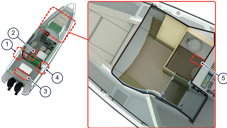
Figure 4.29 - Seacocks
