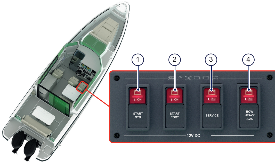
Figure 4.17 - Battery control panel
