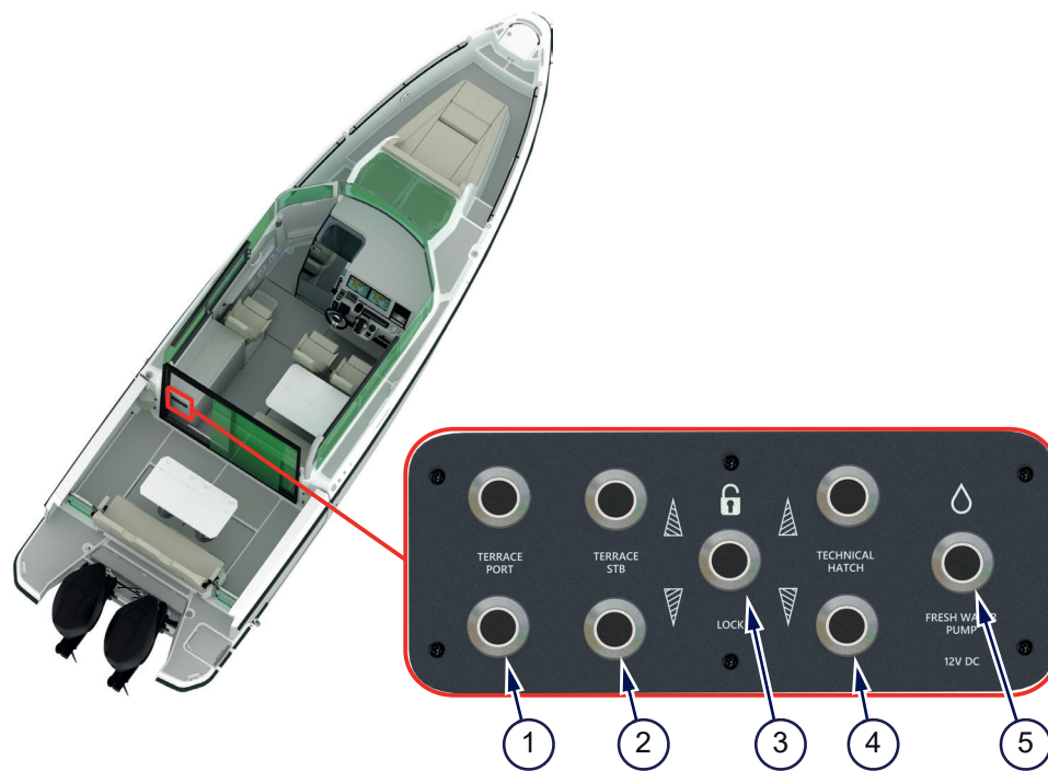
Figure 4.14 - Side terrace control panel
