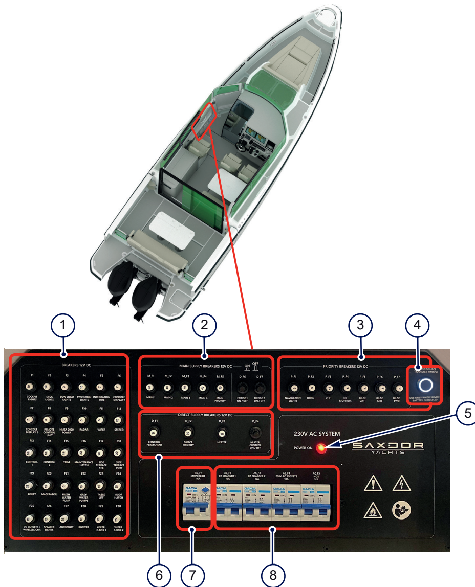
Figure 4.16 - Front cabin fuse panel
