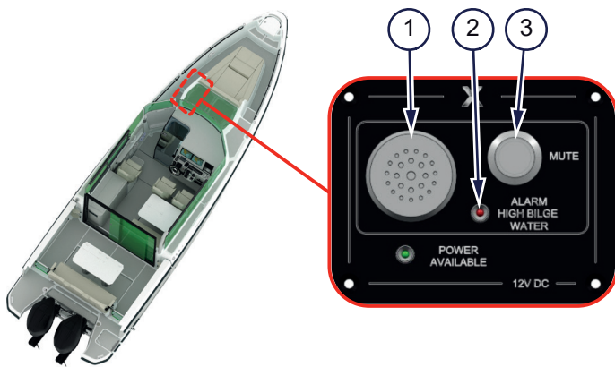
Figure 4.13 - High bilge alarm control panel
