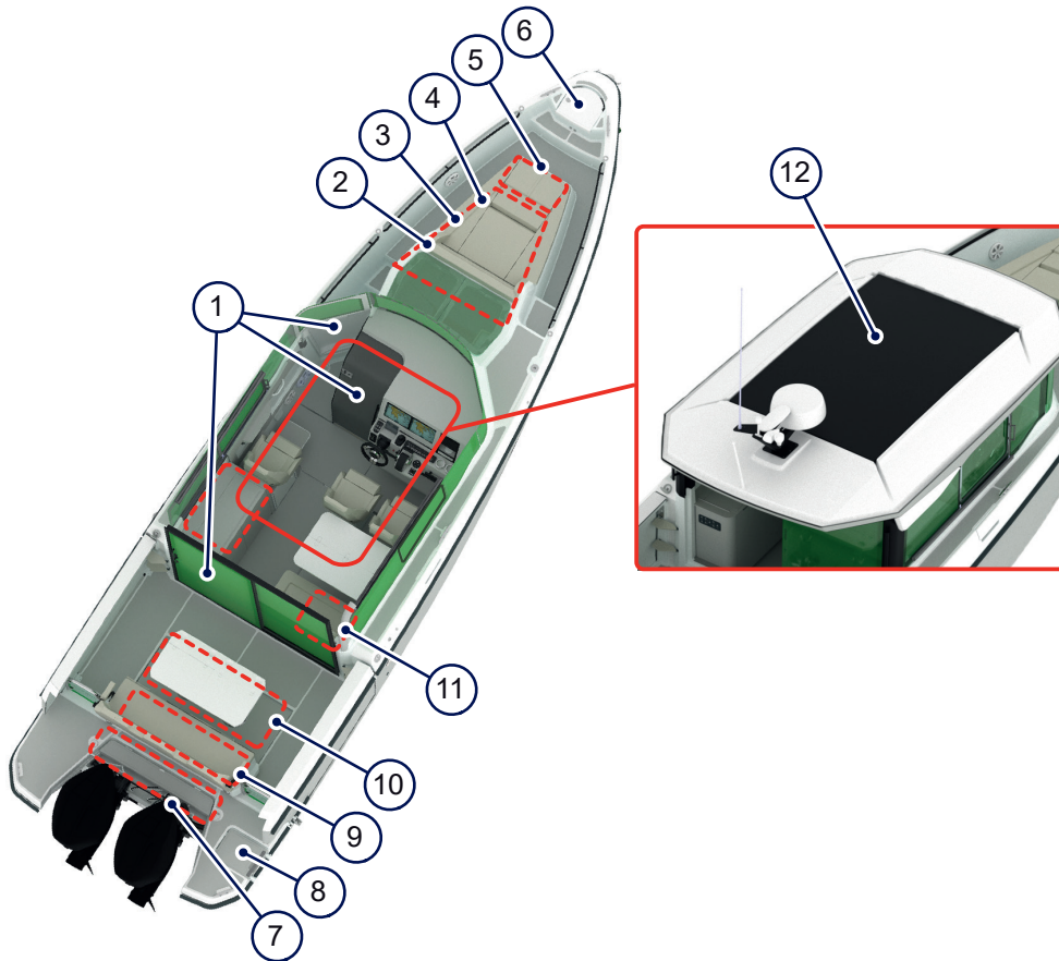
Figure 4.28 - Hatches
