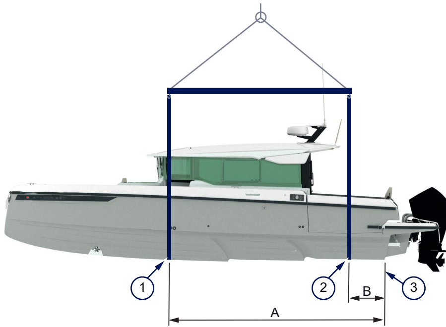
Figure 4.26 - Lifting points
