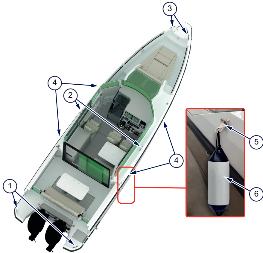
Figure 4.25 - Attachment points
