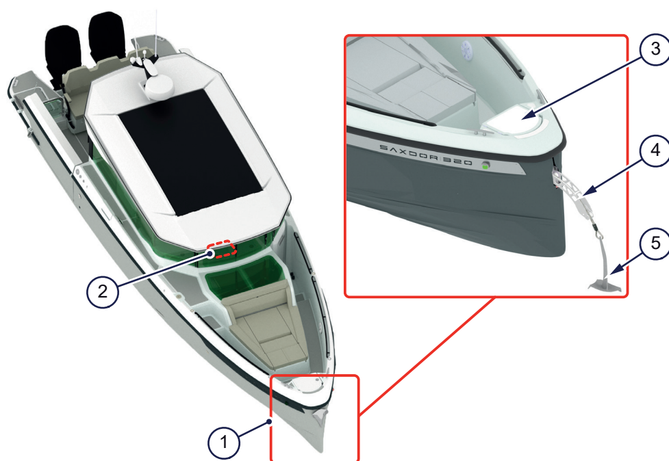
Figure 5.10 - Anchor system
