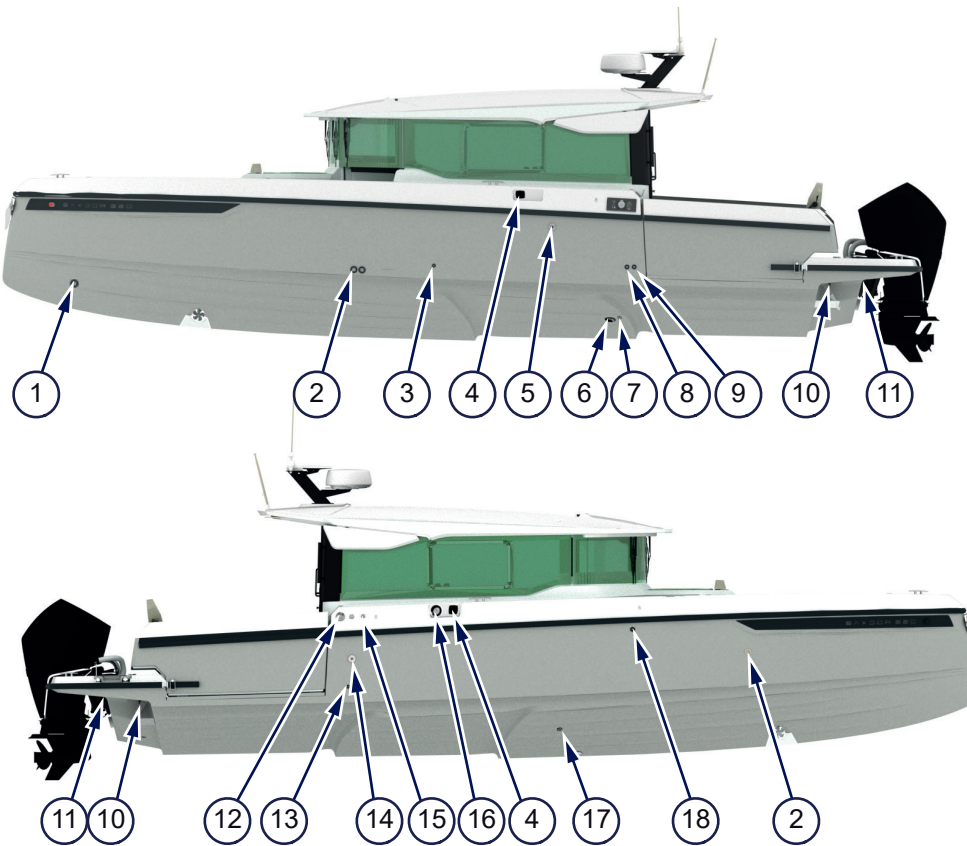
Figure 4.27 - Hull openings
