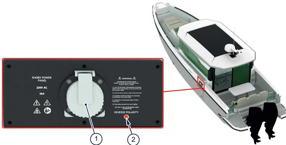
Figure 4.18 - Shore power panel
