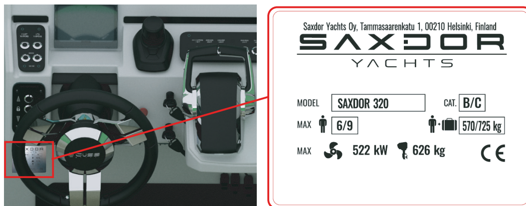
Figure 4.21 - Builder's plate
