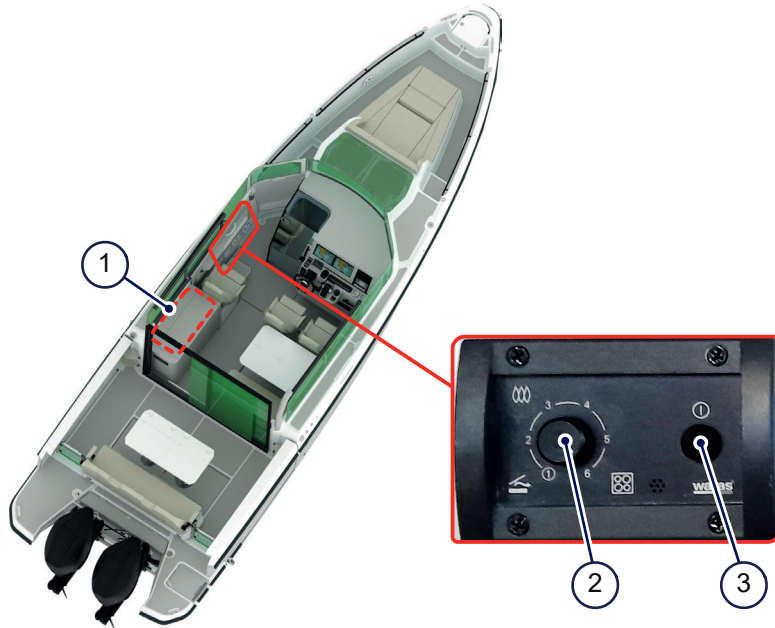
Figure 4.19 - Cooktop control panel
