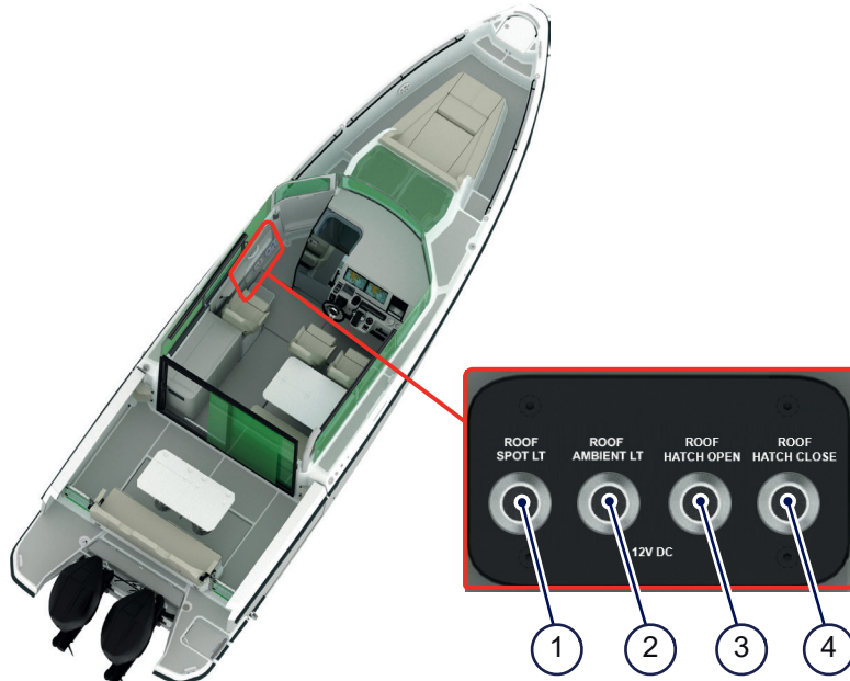
Figure 4.15 - Roof control panel
