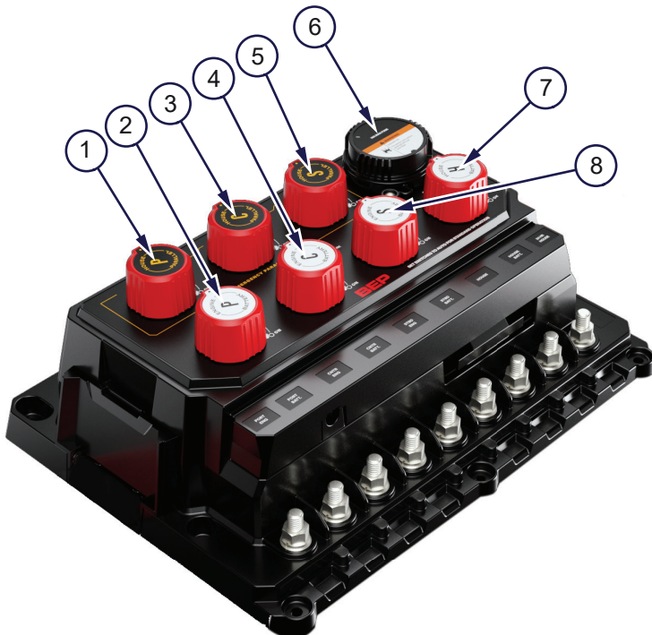
Figure 5.2 - Battery hub
