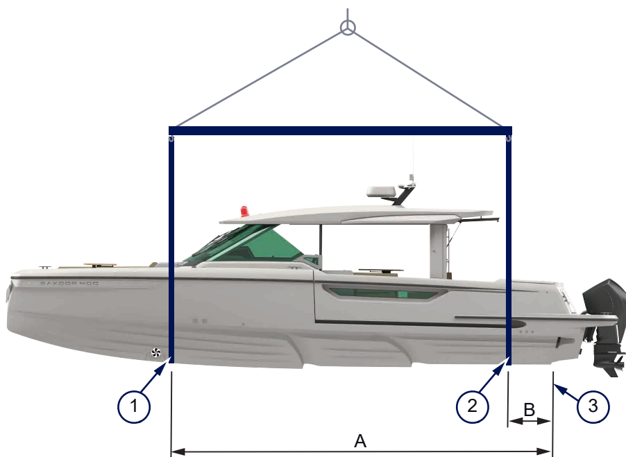
Figure 4.25 - Lifting points
