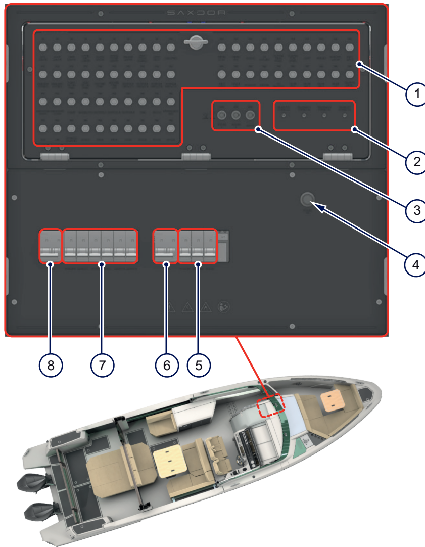
Figure 4.15 - Fuse panel
