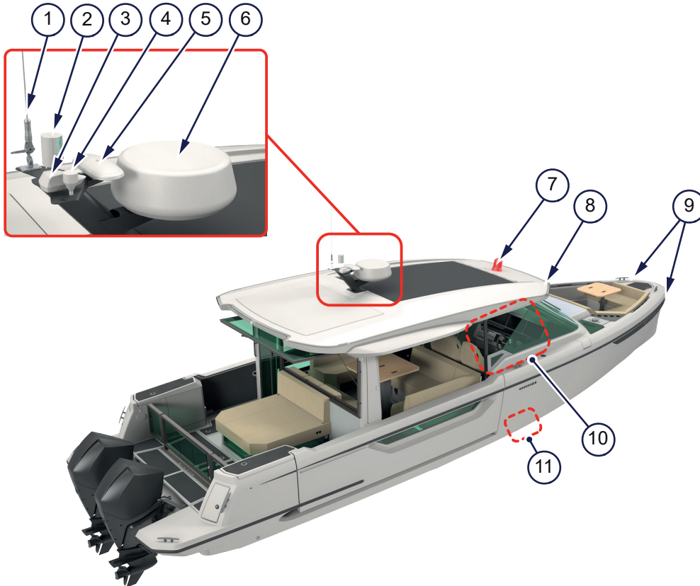
Figure 5.9 - Navigation equipment
