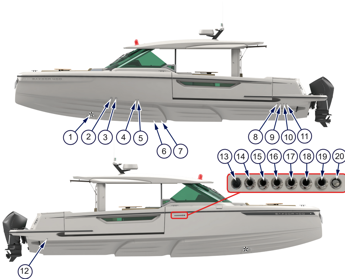
Figure 4.26 - Hull openings
