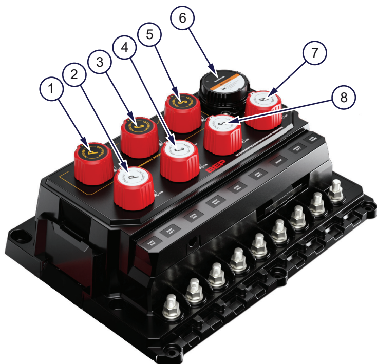
Figure 5.2 - Battery hub
