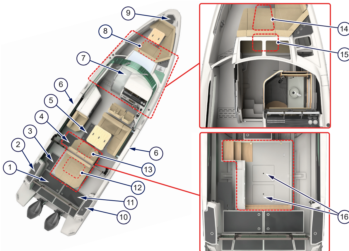
Figure 4.27 - Hatches
