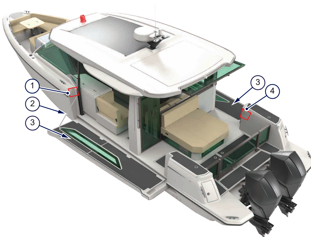
Figure 5.12 - Side terraces
