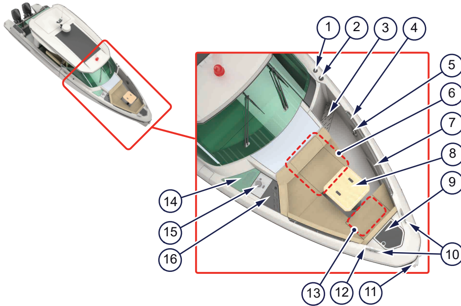
Figure 4.2 - Foredeck
