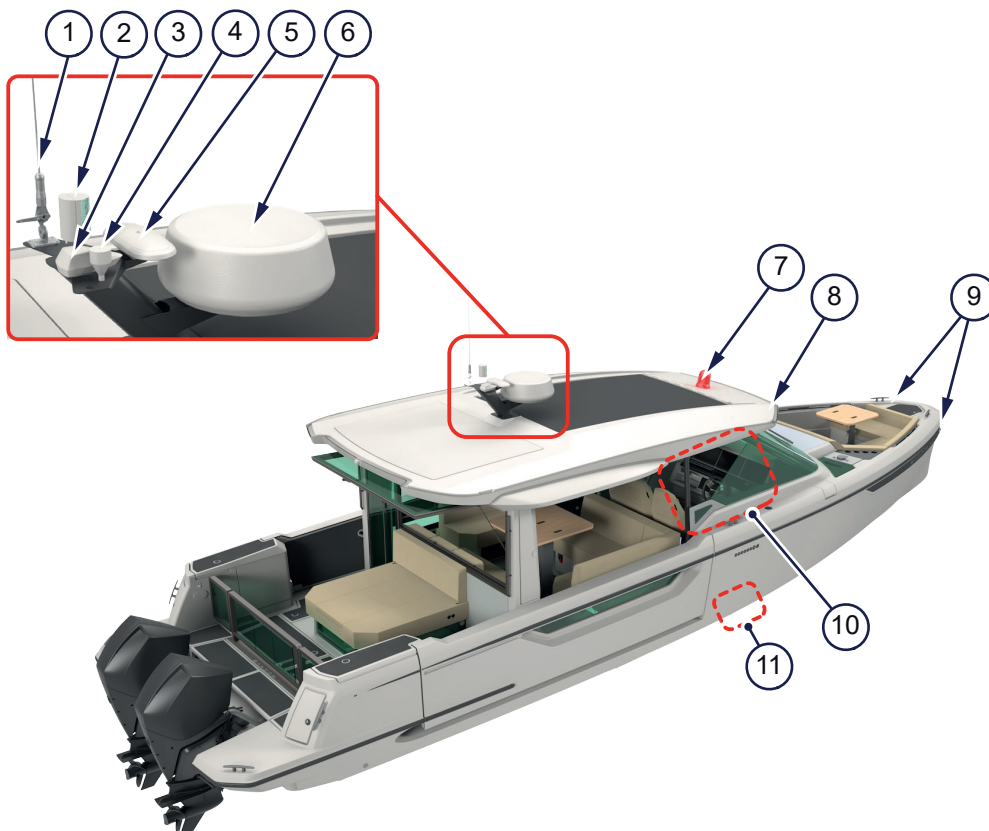
Figure 5.9 - Navigation equipment
