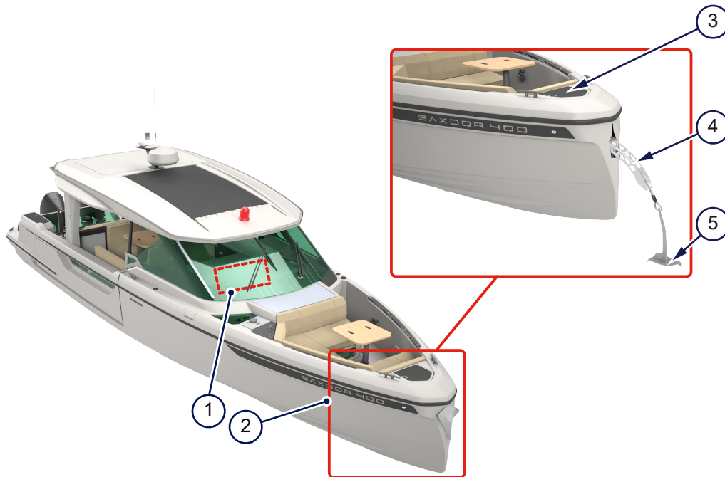
Figure 5.10 - Anchor system
