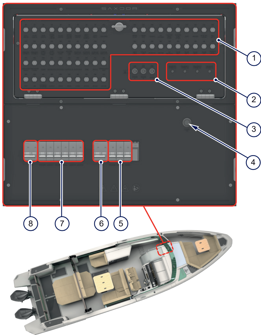
Figure 4.15 - Fuse panel
