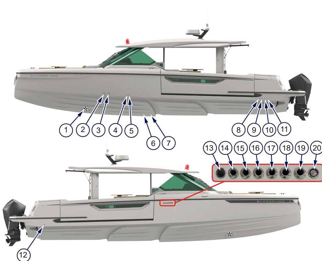
Figure 4.27 - Hull openings
