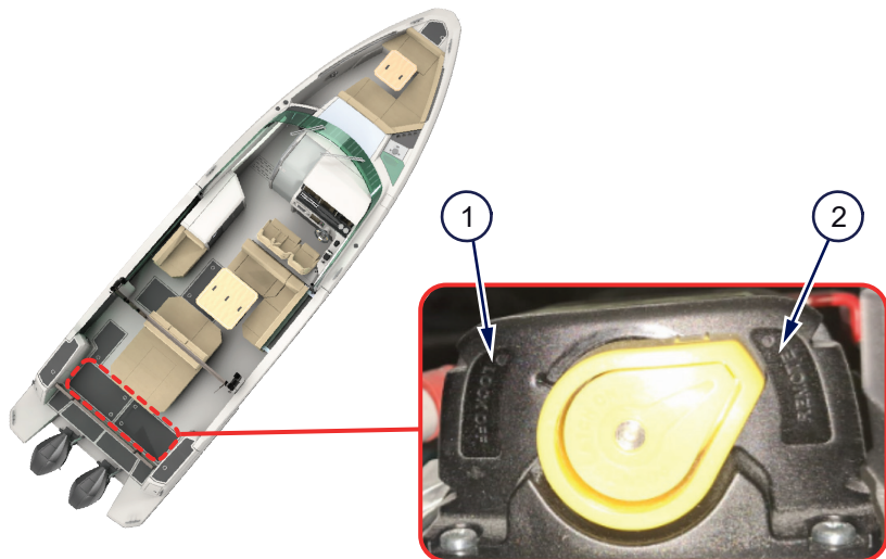
Figure 5.3 - Battery pack safety relay switch
