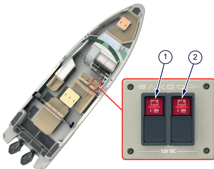
Figure 4.17 - Battery control panel
