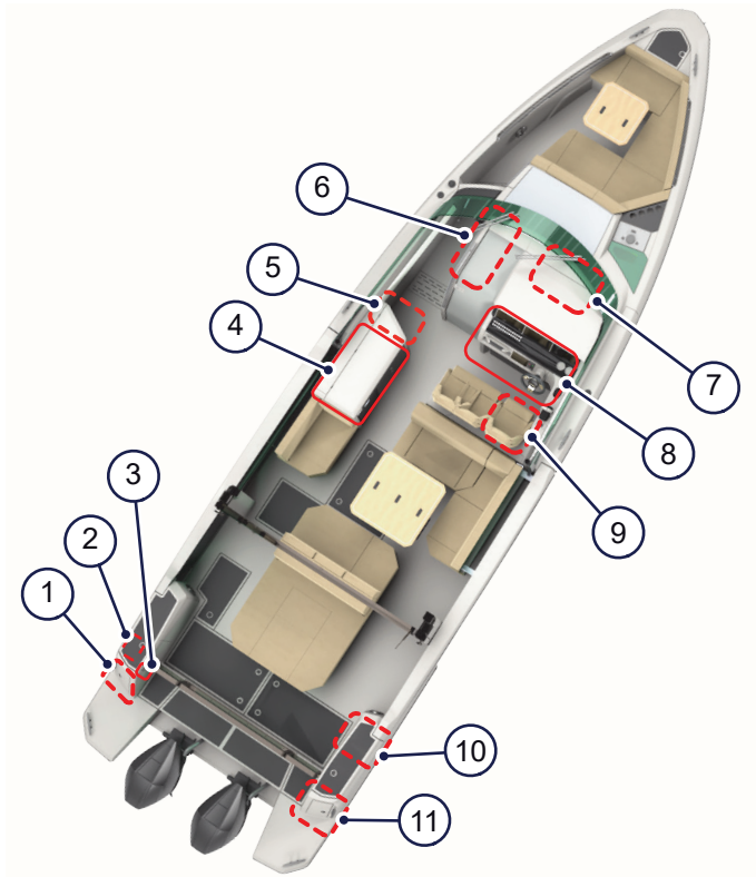
Figure 4.8 - Locations of user controls
