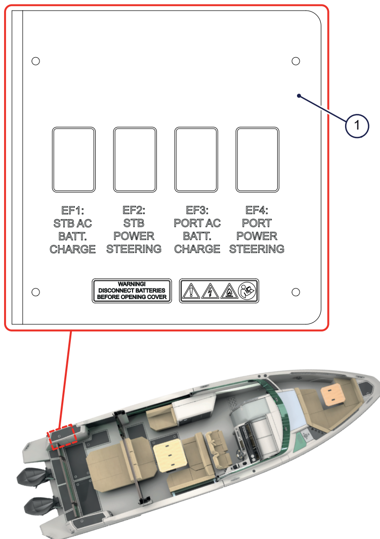
Figure 4.16 - Heavy-duty fuse panel
