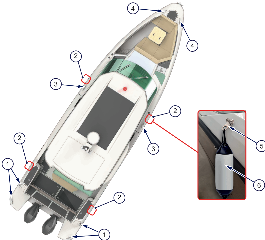
Figure 4.25 - Attachment points
