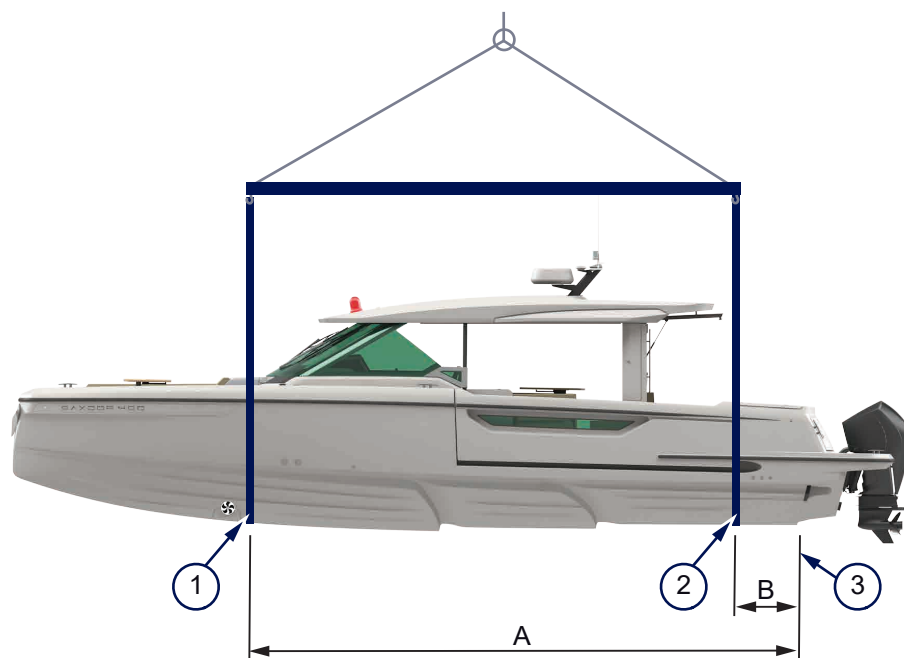
Figure 4.26 - Lifting points
