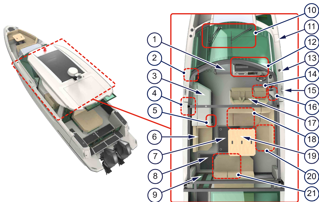
Figure 4.4 - Cockpit
