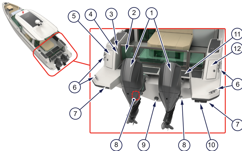
Figure 4.7 - Bathing platform
