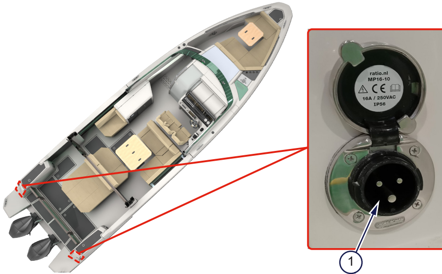
Figure 4.18 - Shore power panel
