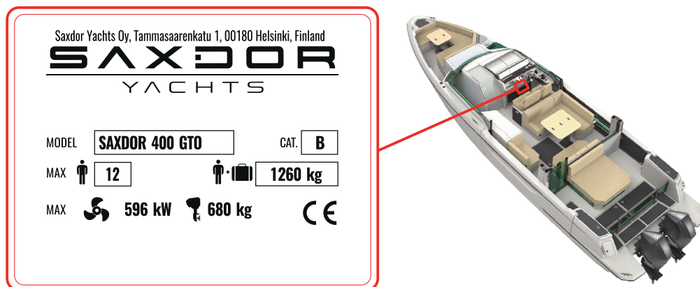
Figure 4.21 - Builder's plate
