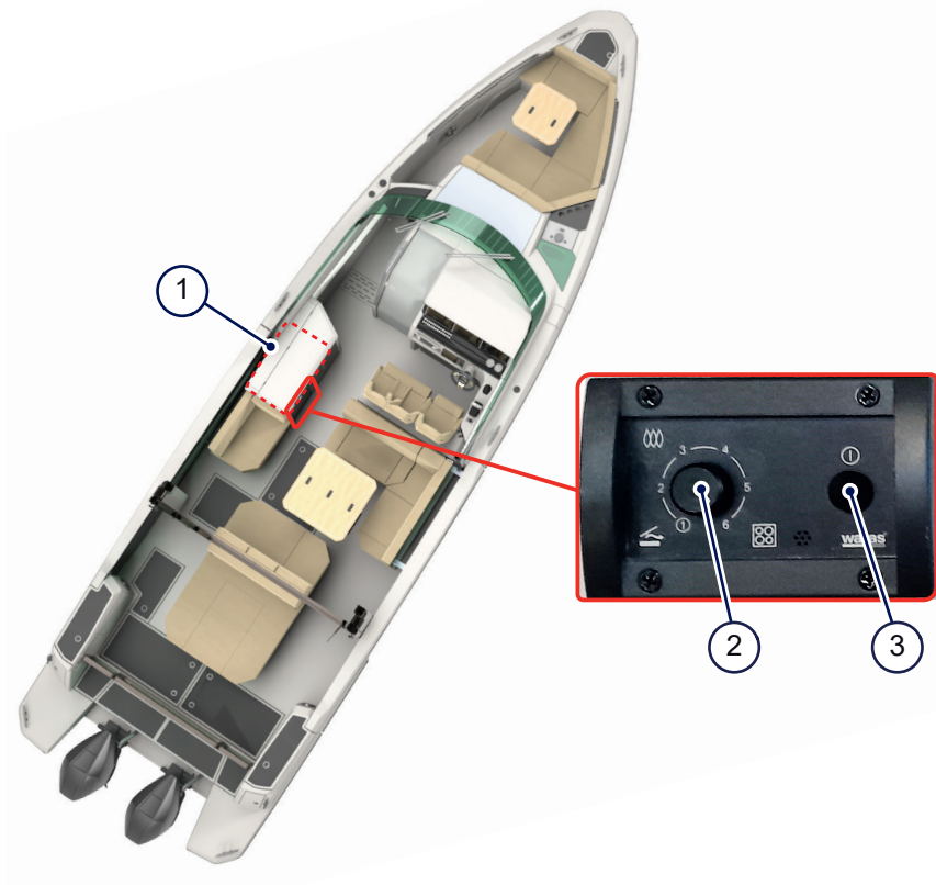
Figure 4.19 - Cooktop control panel
