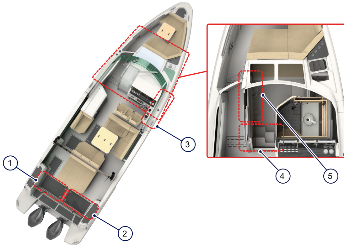
Figure 4.29 - Seacocks
