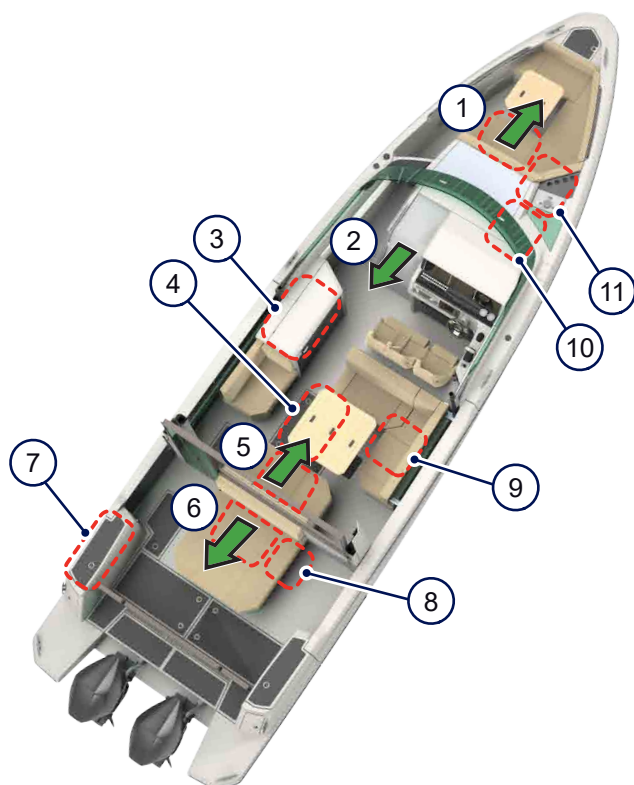
Figure 4.22 - Safety equipment and emergency exits
